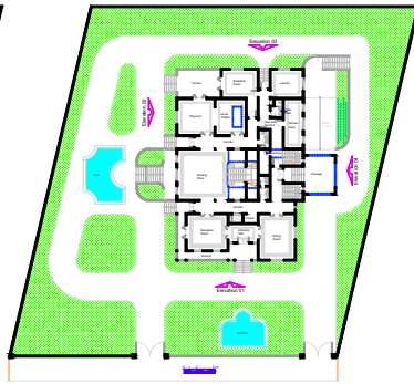
First Floor Plan A = 365,72 m 2
