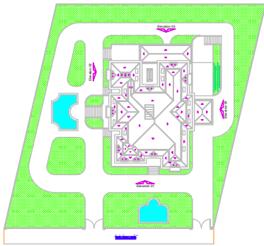
Roof Plan
