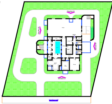
Lower Floor Plan A = 375,35 m 2
