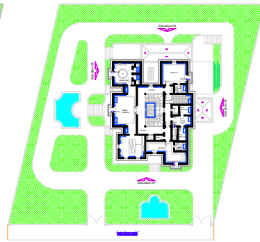
Third Floor Plan A = 260,79 m 2
